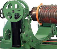
Armature Reroll
