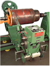
Wire Banding
